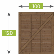
1173 Bramka azur 100x120 R35x70 L5x68 Jalousie screen gate 100x120 F35x70 Portillon ajouré 100x120 C35x70 L5x68 Lamellenzaun für Jalousie 100x120 R35x70
