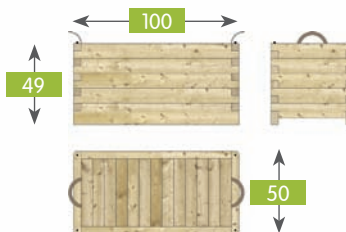
240206B007OMBZ04A1 967 Kwietnik 100x49x50 ram wr R45x90 Flower box 100x49x50 F45x90 Bac 100x49x50 C45x90 Pflanzkasten 100x49x50 R45x90
