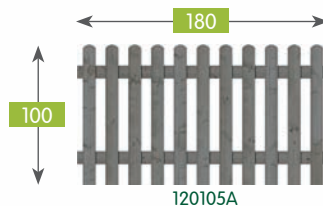
120105A 1322 SZT 180x100 D22x90-11 R22x90 profil B Pale fence 180x100 P22x90-11 profile B Panneau dri 180x100 Staketenzaun 180x100 S22x90-11 R22x90 Profil B jasny szary / bright grey / gris claire / hellgrau
