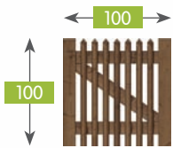
1207 Bramka prosta tocz 100x100 ostrz 55 Straight gate turned 100x100 pointed 55 Portillon droit rond 100x100 app 55 Senkrechtzauntür gek 100x100 gesp 55
