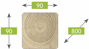
650 190105A012AACZ55A1 Krawędziak 90x90x800 SF rf drob x4 Post 90x90x800 PC small gr x4 Poteau 90x90x800 RC rain fine x4 Kantholz 90x90x800 geh gefast fein geriff x4
