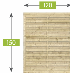
187 Lamela 120x150 R35x55 L4,2x60-64 Screen 120x150 F35x55 Paravue tressé 120x150 C35x55 Lamellenzaun 120x150 R35x55
