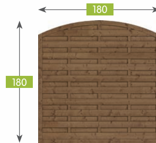
1163 Szczelny Łuk 180x180 R40x60 L7x95 g 3s T screen arch 180x180 F40x60 L sm 3s Panneau stable arc 180x180 C40x60 L li Dichtzaun B 180x180 R40x60 L gl 3S
