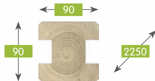
191401A002AACZ52A1 735 Krawędziak H36 90x90x2250 SF Post H36 90x90x2250 PC Poteau H36 90x90x2250 RC Kantholz H36 90x90x2250 geh gefast
