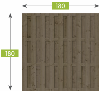
121600A 1318 HOL 180x180 D12x120-17 R19x68-4 Plank fence 180x180 P12x120-17 Panneau planche DRT 180x180 Bretterzaun 180x180 B12x120-17 R19x68-4 ciemny szary / dark grey / gris foncé / dunkelgrau
